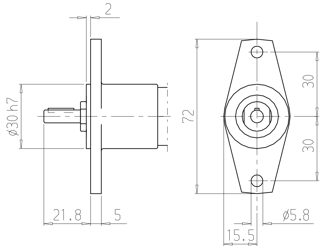
Flange Ordering No. 205 053 6453
