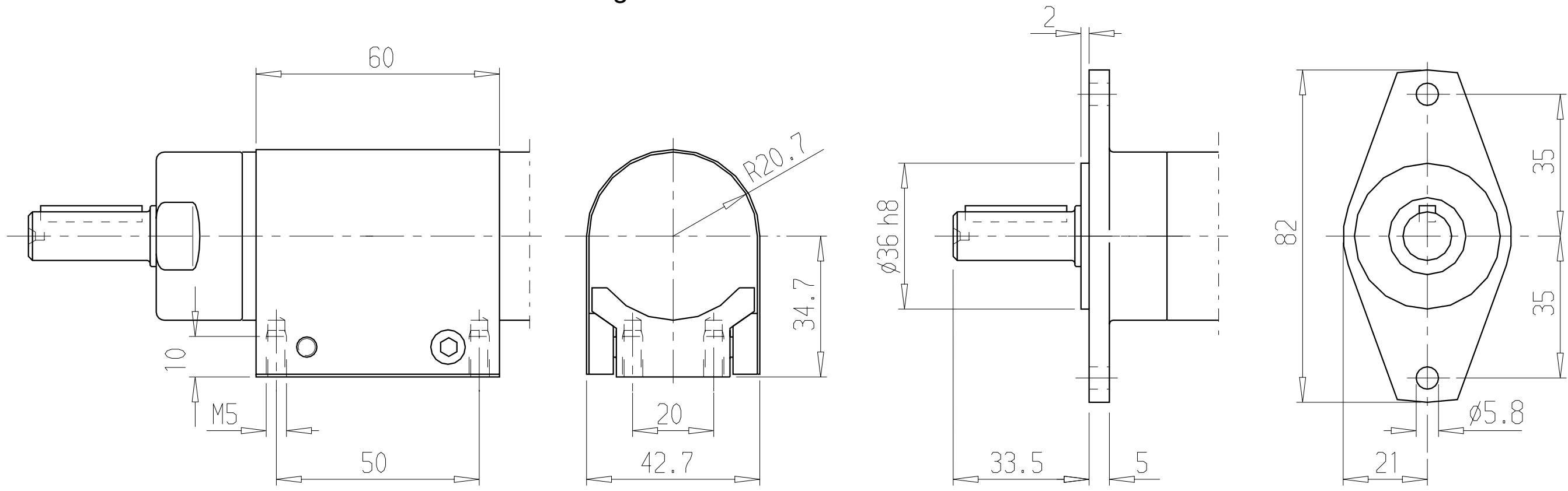
Flange Ordering No. 205 053 6433
